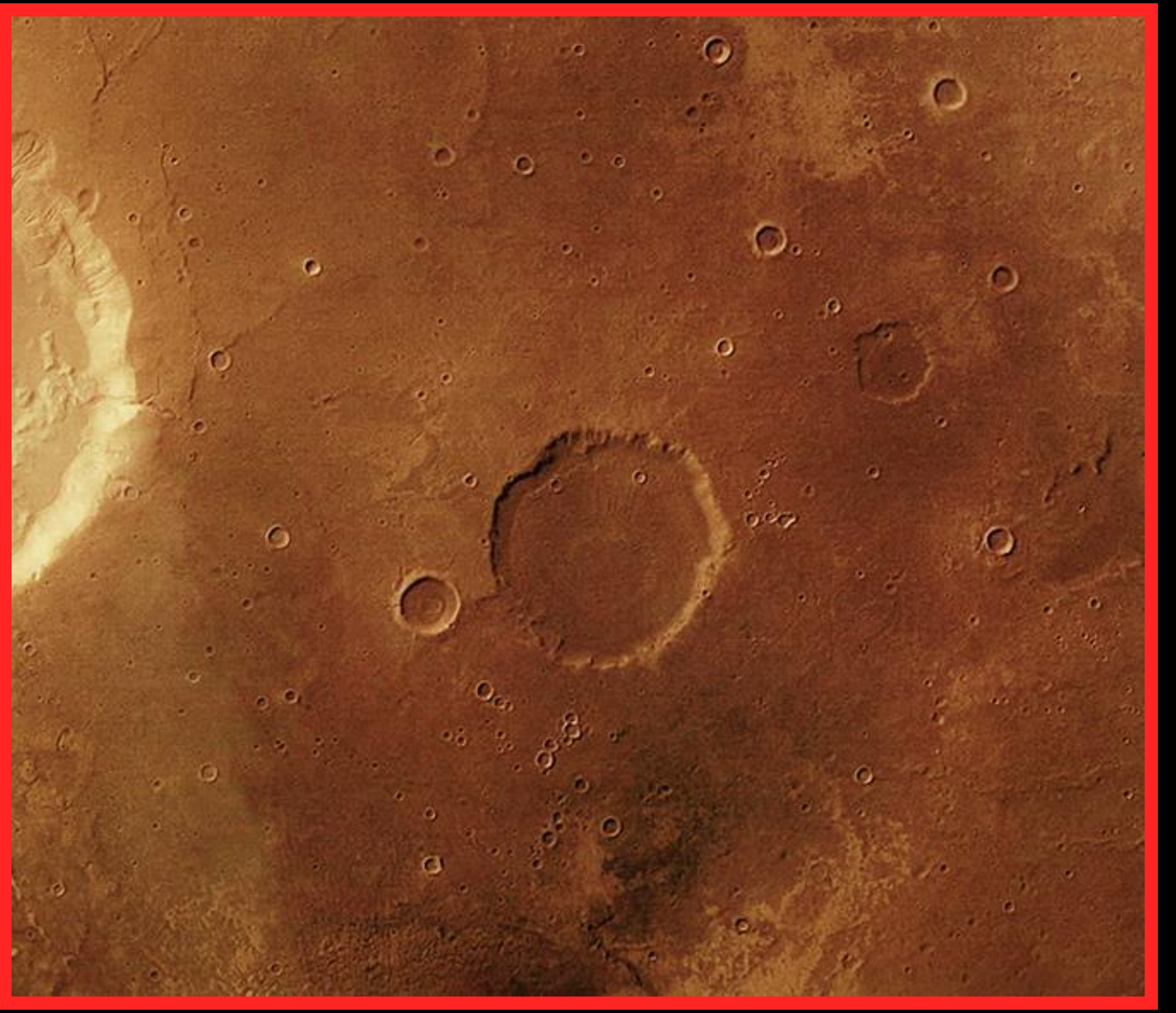
Unnamed impact crater, Arabia Terra
