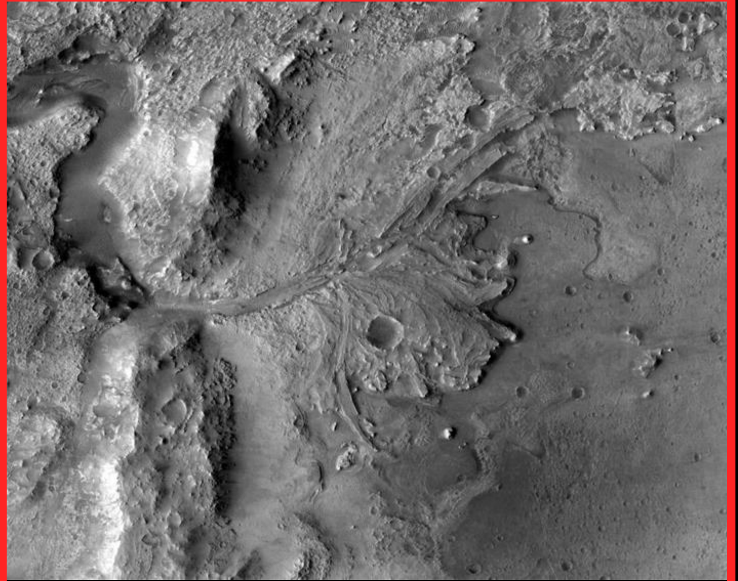
River Delta, Jezero Crater
