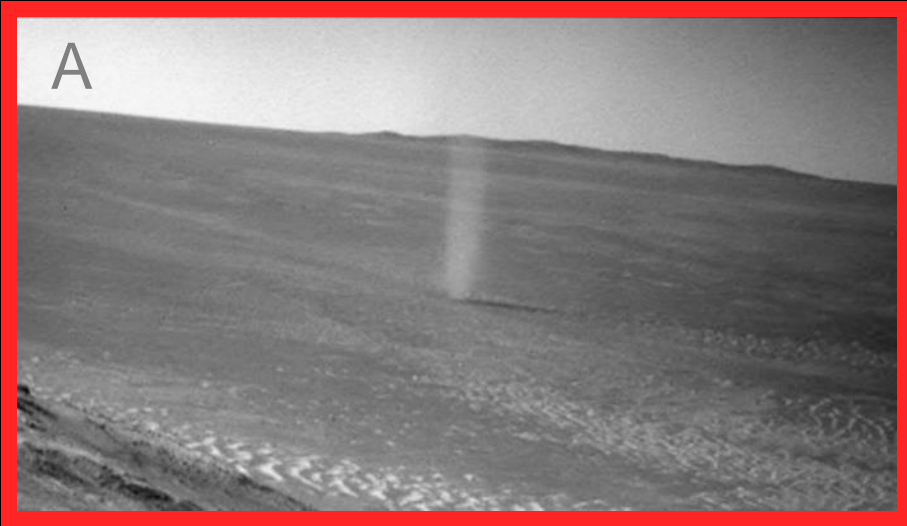
Seen from the ground by the Opportunity rover
