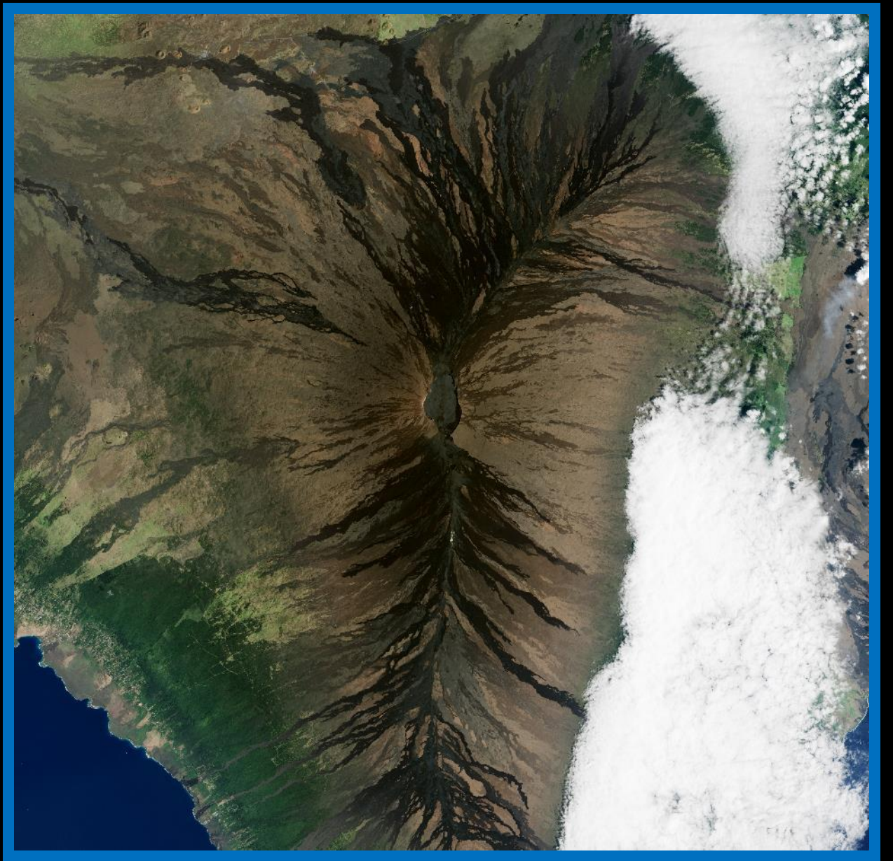
Shield Volcano, Mauna Kea, Hawaii
