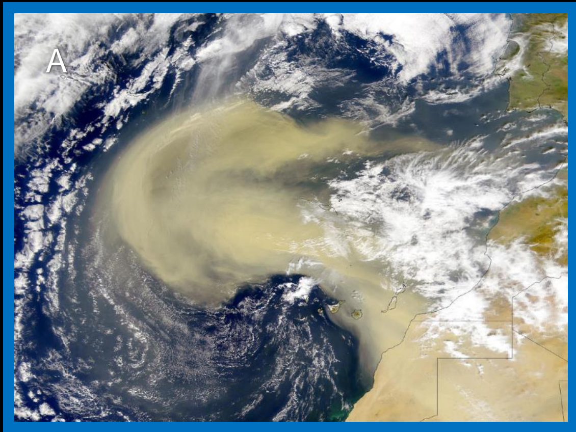
Sahara dust storm
