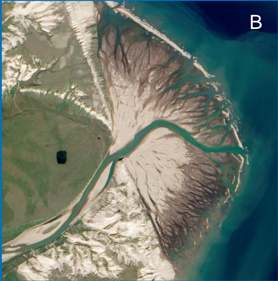
Horton River Delta, Canada
